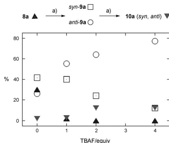
Figure 1. The effect of added Bu 4 NF·3H 2 O (TBAF, 1 M in THF) on the stereoselectivity of the alkylation of 8a . Conditions: a) 8a (0.024 g, 0.152 mmol), [(η 3 -C 3 H 5 )Pd(PPh 3 ) 2 ]BF 4 (5 mol%), NaCH(CO 2 Me) 2 (2 equivalents), [15]crown-5 (2.4 equivalents), TBAF, CH 2 Cl 2 (2 mL), room temperature. Data shown are for 1 H NMR assay of aliquot taken after ten minutes of each run. [14]
